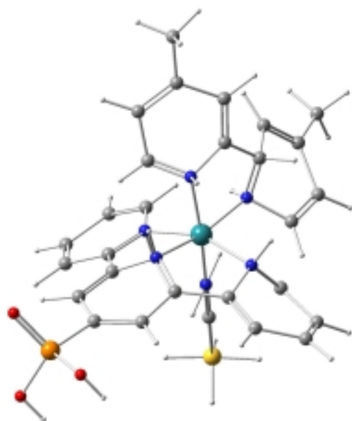
Figure 4: Calculated structure of phosphonated Ru-terpyridine sensitizer synthesised by [13] (a PO 3 group at bottom left, NCS-group bottom mid-behind)
